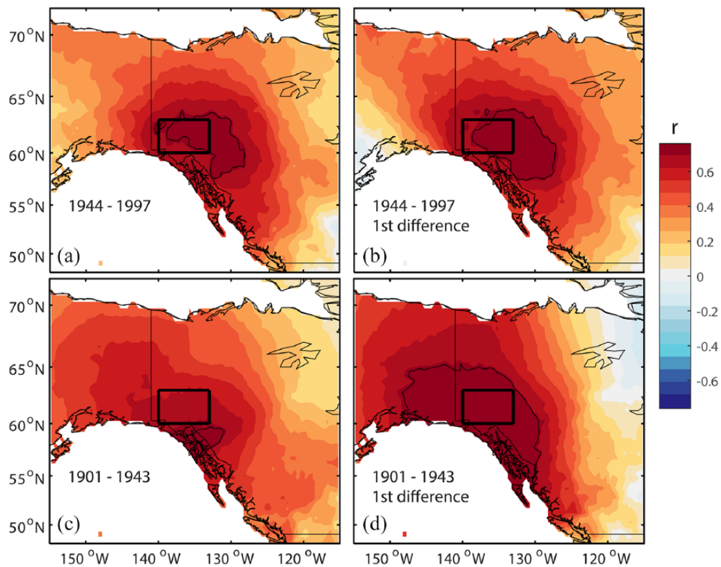
Figure 7. Spatial correlations of ADSne-sf reconstruction with MJJA Tmax for the period 1944–1997 ((a) and (b) are for non-transformed and first differenced correlations) and 1901–1943 ((c) and (d) – as for (a) and (b)). Study region denoted by box while black contour denotes region where r^2 is \geq 0.50 .
